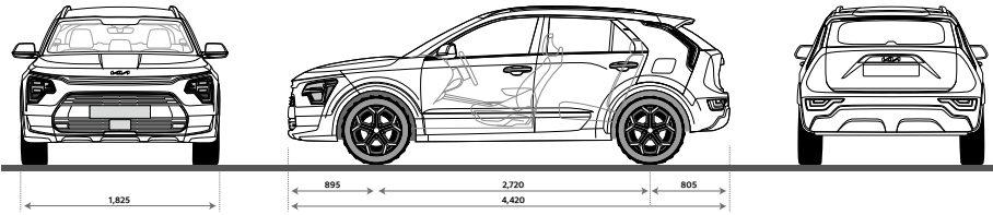
Dimensions HEV (mm)
