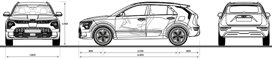
Dimensions EV (mm)
