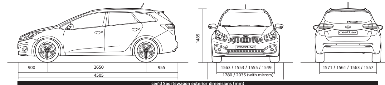
cee'd Sportswagon exterior dimensions (mm)
