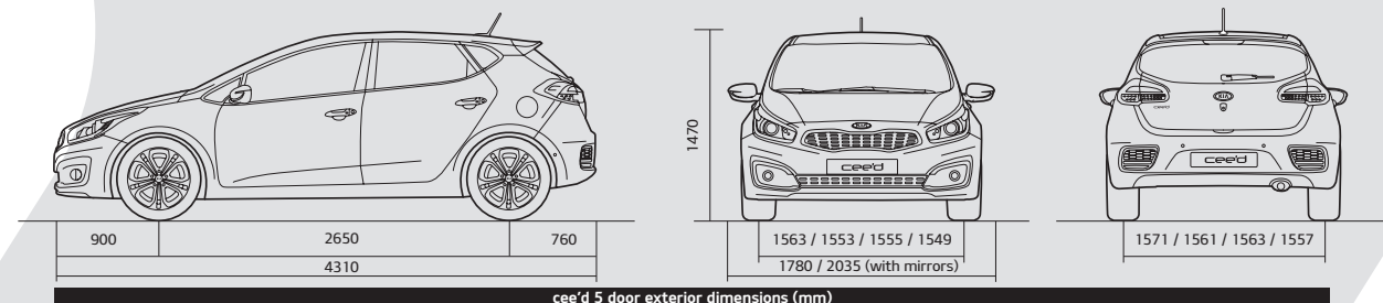
cee'd 5 door exterior dimensions (mm)
